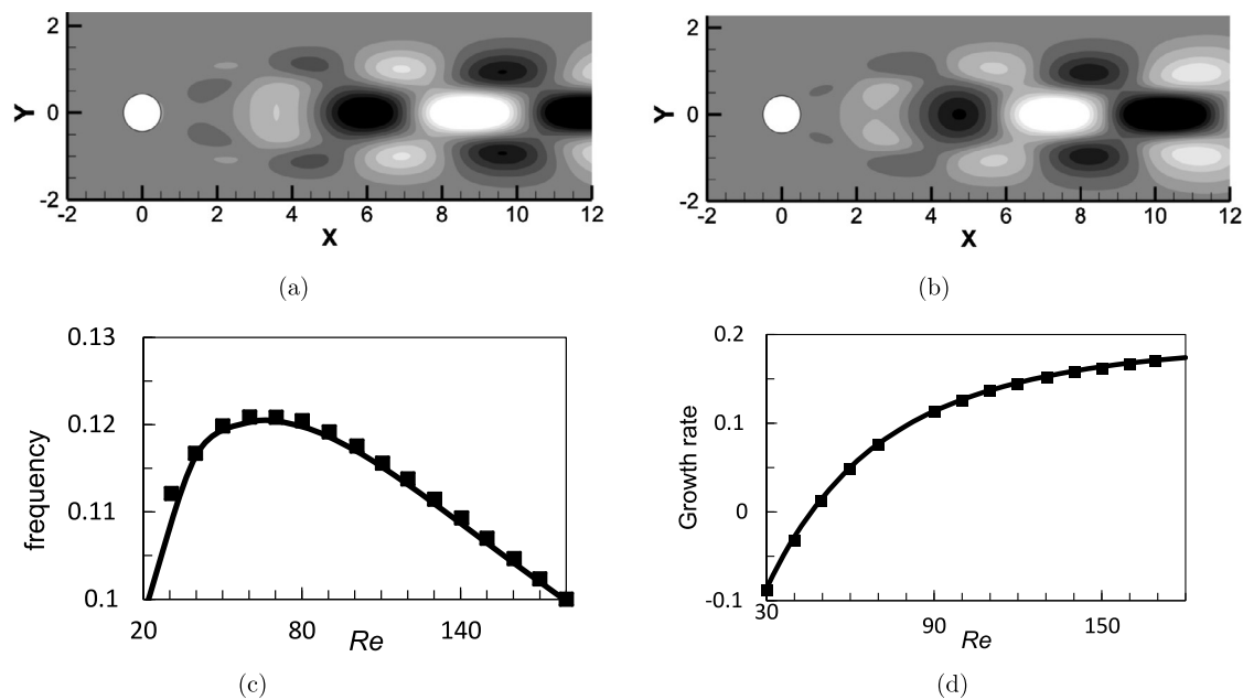
Fig. 9. Results of the linear stability analysis of incident flow over the cylinder at Re = 100 : (a) real part of the leading eigenmode of vorticity; (b) imaginary part of the leading eigenmode of vorticity; (c) comparison of the critical frequency values (bold line) obtained in this study with the reference values (black squares, scanned from [56]) as a function of the Re number; (d) comparison of the growth rate values (bold line) obtained in this study with the reference values (black squares, scanned from [56]) as a function of the Re number.
