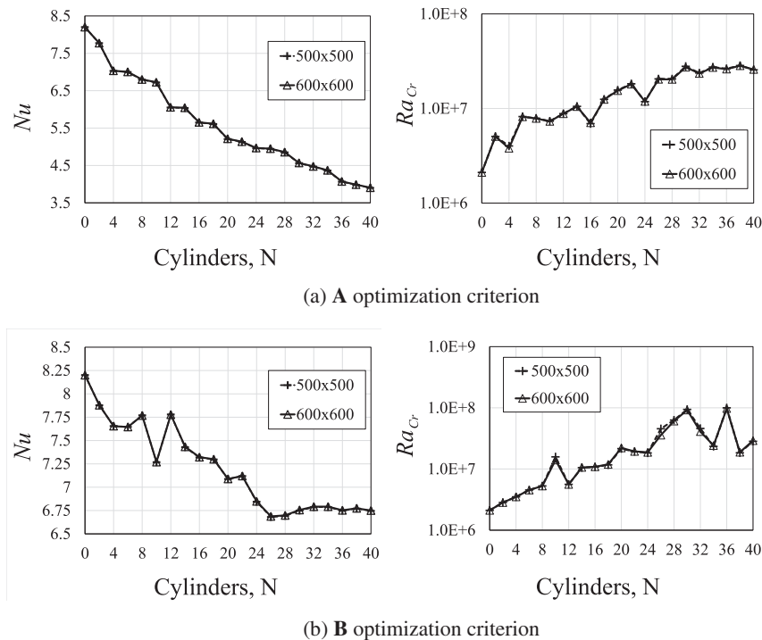
Fig. 6. Variation of the values of the averaged Nu number obtained for the vertical hot wall of the cavity at Ra_0 = 2.11 \times 10^6 and the critical Rayleigh number, Ra_{cr} for the steady-unsteady transition obtained by the linear stability analysis as a function of the number of cylindrical obstacles for: (a) A optimization criterion; (b) B optimization criterion. The calculations were performed on 500 \times 500 and 600 \times 600 grids.
