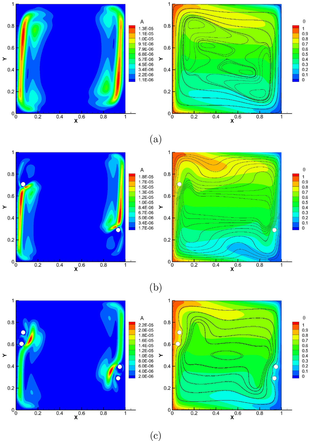
Fig. 4. Contours of criterion A and the corresponding steady state distribution of the temperature, \theta with superimposed streamlines obtained at Ra_{cr}^0 = 2.11 \times 10^6 for: (a) no obstacles; (b) 2 obstacles; (c) 4 obstacles; (d) 6 obstacles; (e) 8 obstacles; (f) 10 obstacles; (g) 20 obstacles; and (h) 40 obstacles. The diameter of all the obstacles is equal to d=0.04 .
