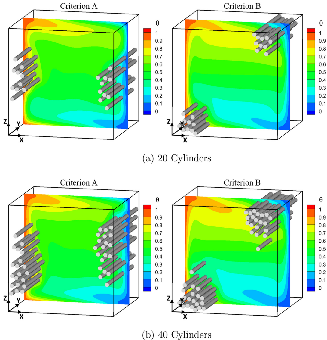
Fig. 7. 3D setup obtained by extension of the corresponding 2D configurations in the z direction with a superimposed temperature distribution at the mid cross-section of the cavity obtained at Ra=2.11 \times 10^6 by: (a) 20 cylinders, the location of which was obtained by utilizing optimization criteria A and B ; and (b) 40 cylinders, the location of which was obtained by utilizing optimization criteria A and B .
