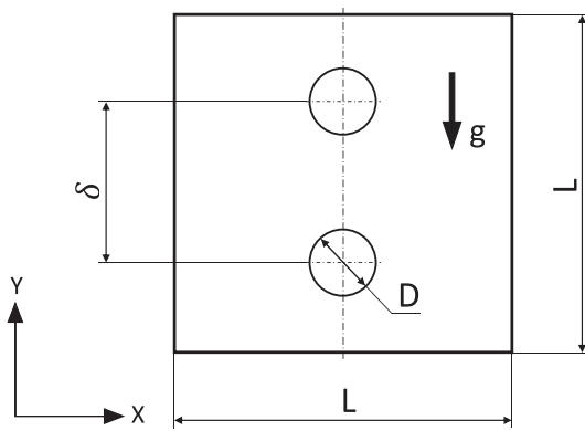
Fig. 2. Schematic representation of a geometrical model of the computational domain showing vertically aligned cylinders confined in a square cavity. Arrow indicates the direction in which the force of gravity acts.
